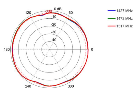
Azimuth: 1427 – 1517 MHz
