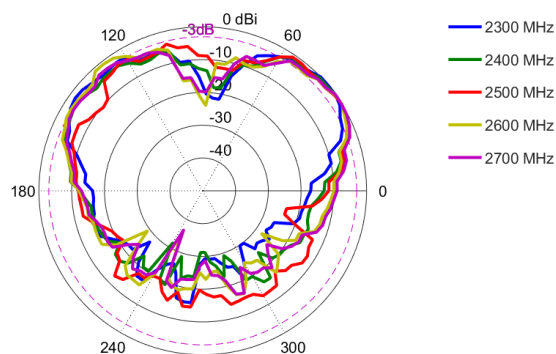
Azimuth: 2300 – 2700 MHz
