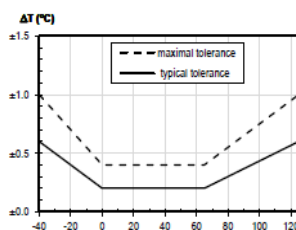
Figure 1 Temperature accuracy
