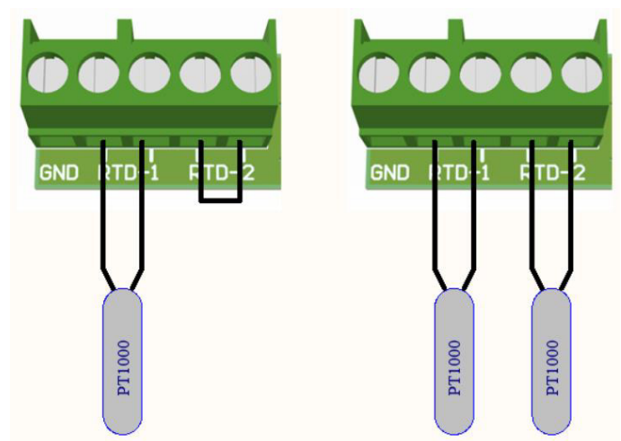
Connection of one PT1000
