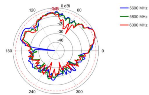
Elevation 2: 5600 – 6000 MHz
