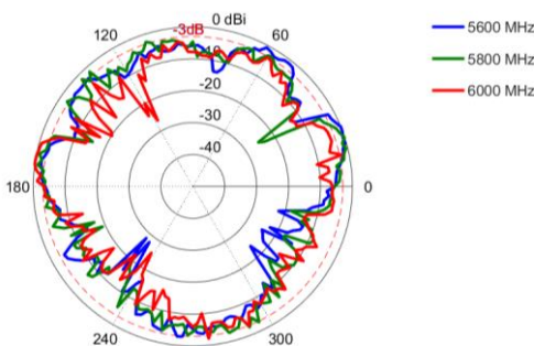
Elevation 1: 5600 – 6000 MHz
