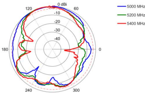
Elevation 2: 5000 – 5400 MHz
