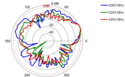
Elevation: 5000 – 5400 MHz
