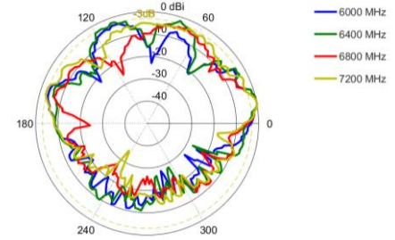
Elevation: 6000 – 7200 MHz
