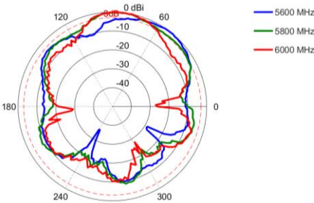
Azimuth: 5600 – 6000 MHz
